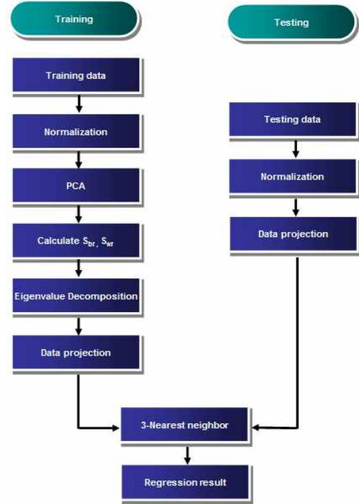
Fig. 2. Flowchart of regression process using LDAR.
