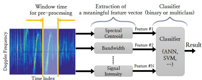
Fig. 1. The example of the conventional approach for classification of human walking. It requires complicated processes such as statistical analysis which is considered as a heuristic method in order to extract a meaningful and effective feature vector.
